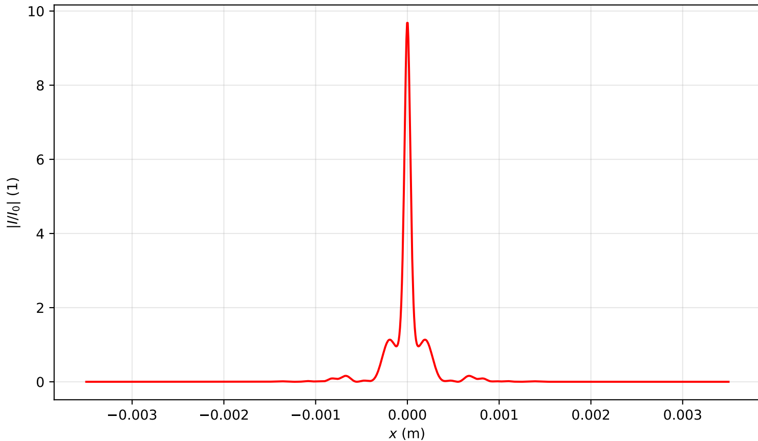
Intensity profile I(x, y = 0, z = 0.955)/I_0 , \text{Pin}=7.0\text{Pcr} , artificial time
